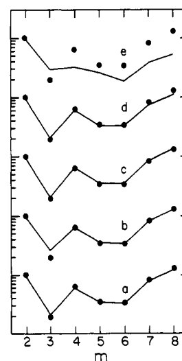
Figure 2. Higher order potential constants (\partial^m V / \partial \tilde{S}_{t2}^m) / m! divided by the quadratic constant, for t_2 symmetry coordinate \tilde{S}_{t2} = (\tilde{S}_{4x} + \tilde{S}_{4y} + \tilde{S}_{4z}) / 3^{1/2} , logarithmic scale. Points, POS; lines, EHT; for labels, see caption of Figure 1.
