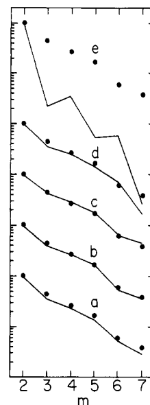
Figure 1. Higher order potential constants [(\partial^m V / \partial \tilde{S}_{2a}^m) / m!] / [(\partial^2 V / \partial \tilde{S}_{2a}^2) / 2] , for e symmetry coordinate \tilde{S}_{2a} , logarithmic scale. Dots, POS field; lines, EHT. Molecular orbital calculations: a, CF 4 ; b, SiF 4 (including d on Si); c, SiF 4 (excluding d); d, CCl 4 ; e, CH 4 . For odd m both POS and EHT constants were negative.
